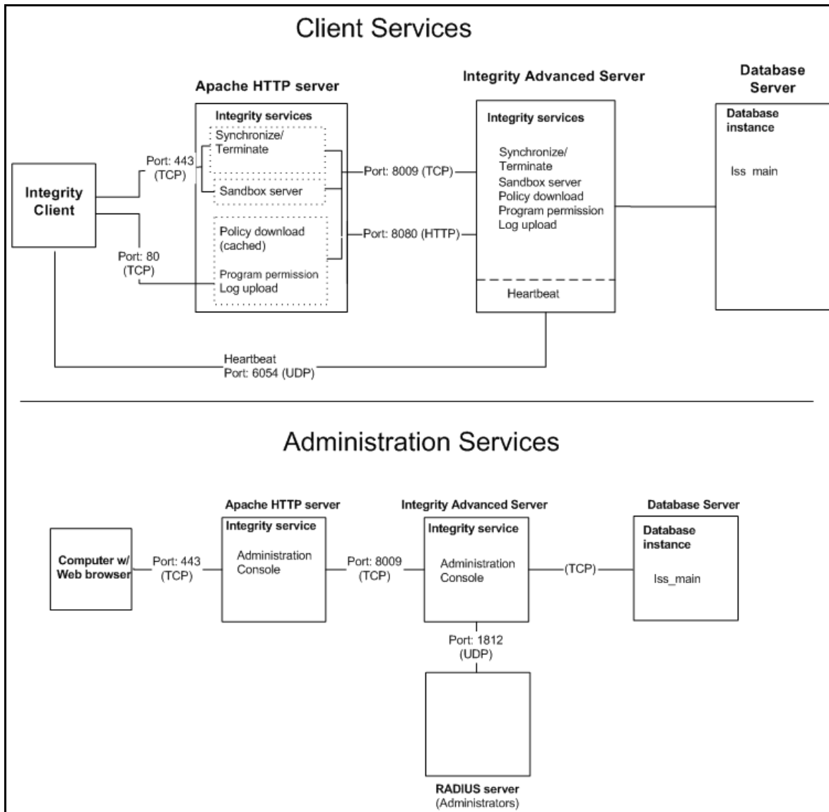
Figure 3-2: Integrity Advanced Server services and ports
