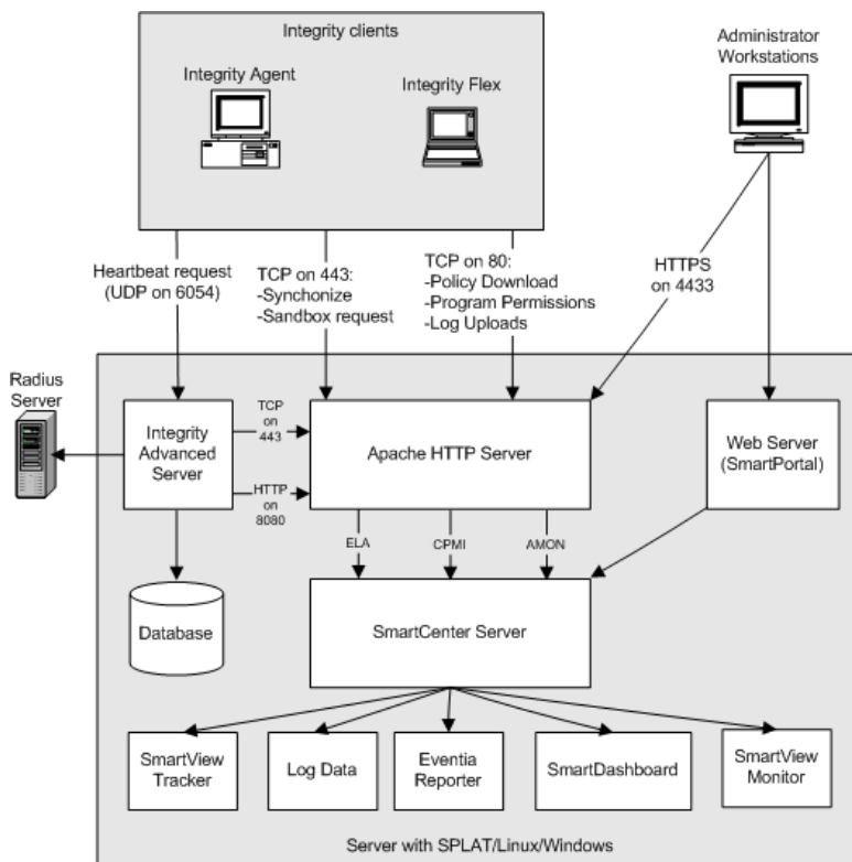
Figure 3-1: typical Integrity Advanced Server Configuration
